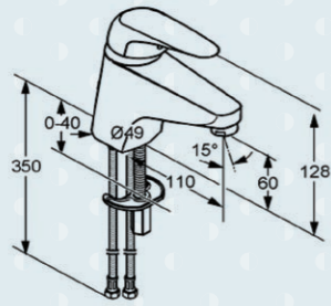
basin mixer product no. 017312
