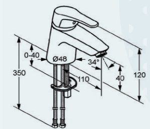
basin mixer product no. 017301
