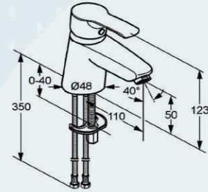
basin mixer product no. 017306
