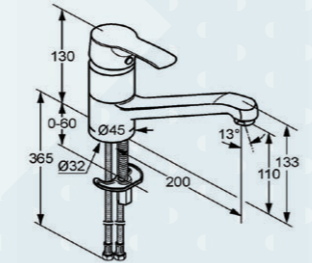
sink mixer product no. 017310
