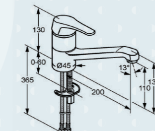
sink mixer product no. 017305
