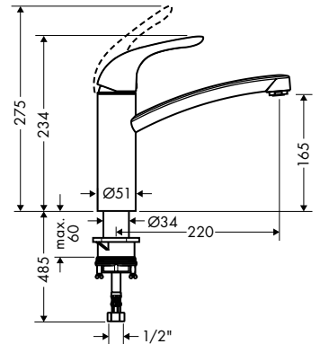
Focus E – Sink Mixer WELS 4★ (7L/min) #109955
