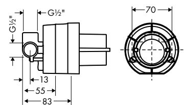
Focus E – Bath/Shower Mixer (body only) #109956
