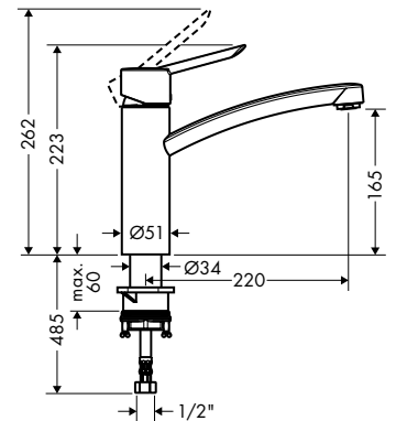
Focus S – Sink Mixer WELS 4★ (7L/min) #109952
