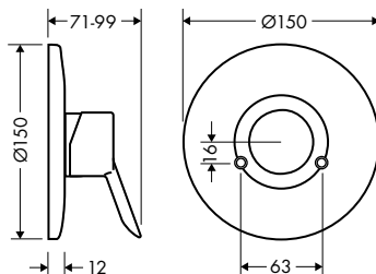
Focus S – Bath/Shower Mixer (trim only) #109951
