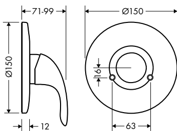
Focus E – Bath/Shower Mixer (trim only) #109954
