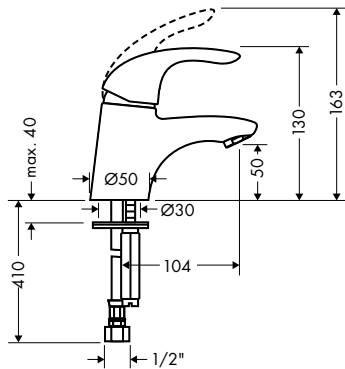
Focus E – Basin Mixer WELS 4★ (7L/min) #109953
