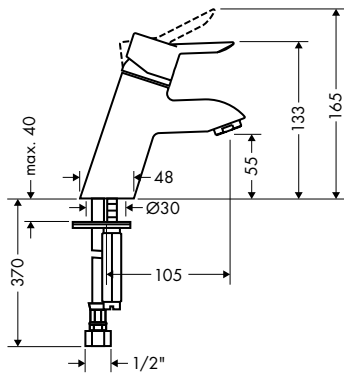
Focus S – Basin Mixer WELS 4★ (7L/min) #109950
