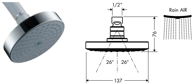
Raindance – S150 1-Jet Shower Head (shower arm not included) WELS 3★ (9L/min) #109961
