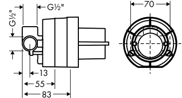
Focus S – Bath/Shower Mixer (body only) #109956
